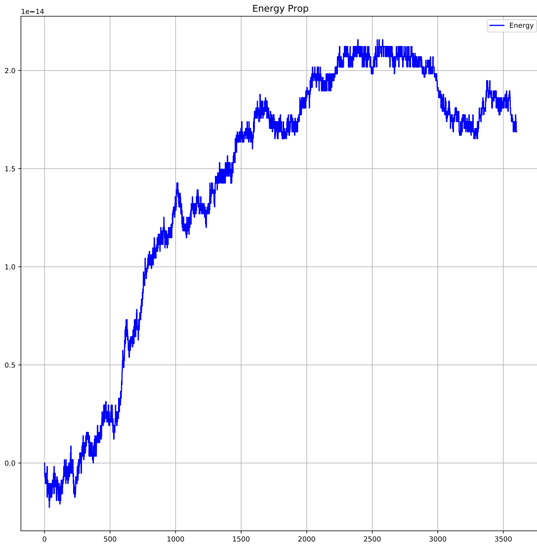
Fig. 1: Orbital Energy
