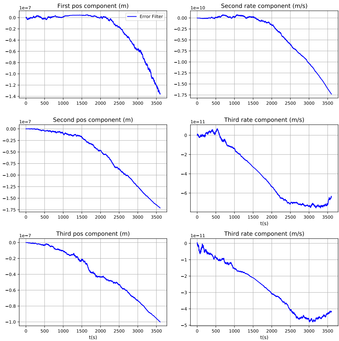
Fig. 2: State error
