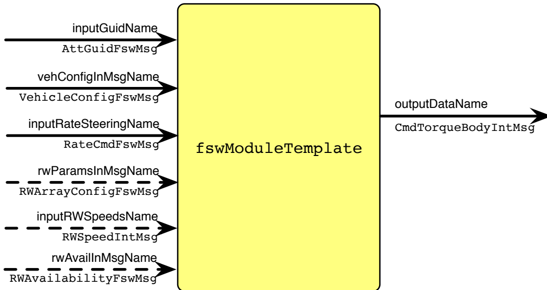
Fig. 1: reateServoFullNonlinear Module I/O Illustration
