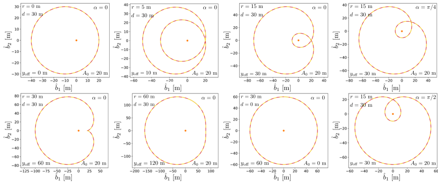
Fig. 5 Bounded body-frame relative trajectory for a circular chief orbit with constant and resonant orbit-normal spin motion. The solid red curve is generated from the LROE formulation, while the dashed yellow curve is generated from the equivalent epitrochoid parameterization using the derived shape parameters
