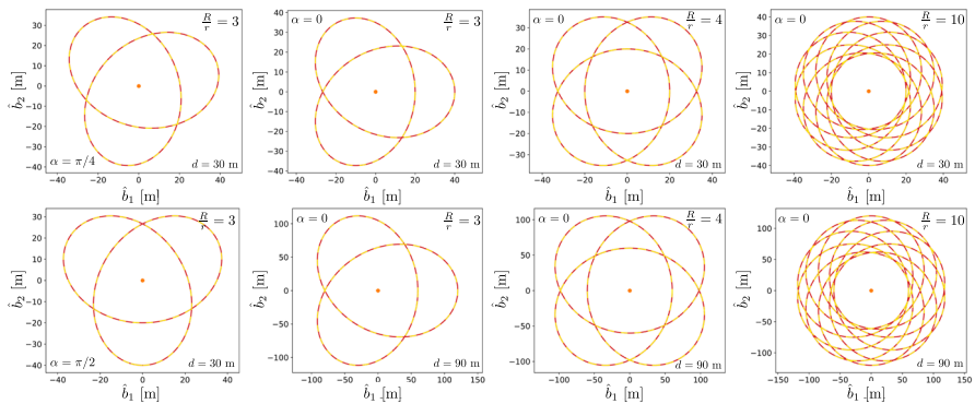
Fig. 8 Bounded body-frame relative trajectory for a circular chief orbit with orbit-normal spin motion, where orbit rate is greater than spin rate. The solid red curve is generated from the LROE formulation, while the dashed yellow curve is generated from the equivalent hypotrochoid parameterization using the derived shape parameters
