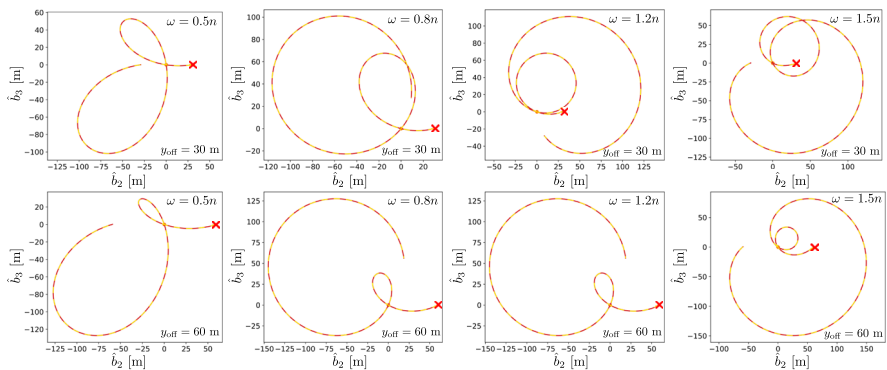
Fig. 13 Body-frame relative trajectory for a circular chief orbit with constant, non-resonant nadir spin. The relative motion in the Hill frame is planar, leading to a time-varying trochoidal pattern in the body frame. The solid red curve is generated from the LROE formulation, while the dashed yellow curve is generated from the equivalent epitrochoid parameterization using the derived shape parameters. The red x marks the trajectory start
