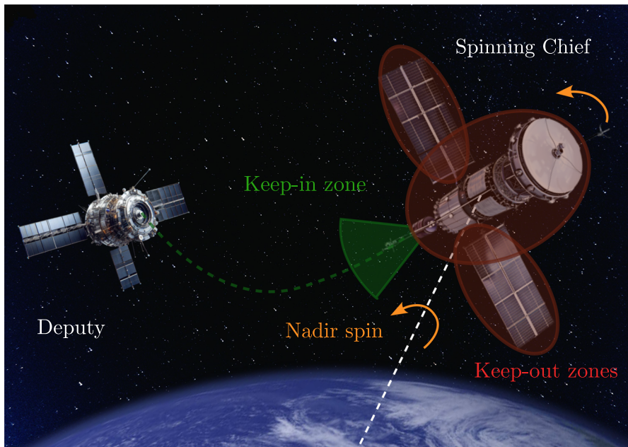
Fig. 1 Concept figure of a servicing mission to a spinning chief
