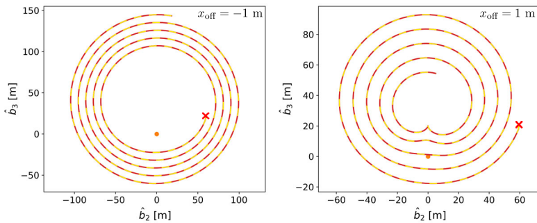
Fig. 11 Unbounded body-frame relative trajectory for a circular chief orbit with constant and resonant nadir spin motion. The solid red curve is generated from the LROE formulation, while the dashed yellow curve is generated from the equivalent epitrochoid parameterization using the derived shape parameters. The red x marks the trajectory start
