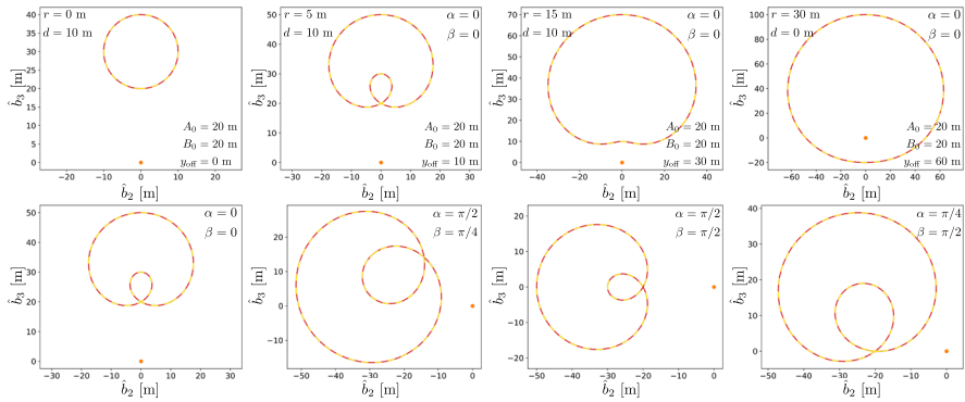
Fig. 10 Bounded body-frame relative trajectory for a circular chief orbit with constant and resonant nadir spin motion. The solid red curve is generated from the LROE formulation, while the dashed yellow curve is generated from the equivalent epitrochoid parameterization using the derived shape parameters
