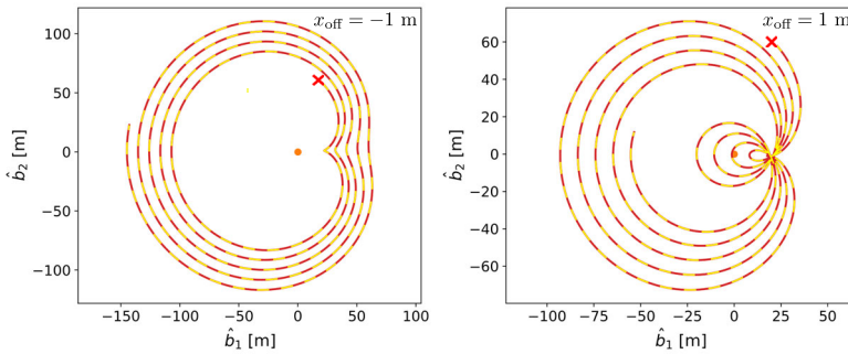
Fig. 6 Unbounded body-frame relative trajectory for a circular chief orbit with constant and resonant orbit-normal spin motion. The solid red curve is generated from the LROE formulation, while the dashed yellow curve is generated from the equivalent epitrochoid parameterization using the derived shape parameters. The red x marks the trajectory start
