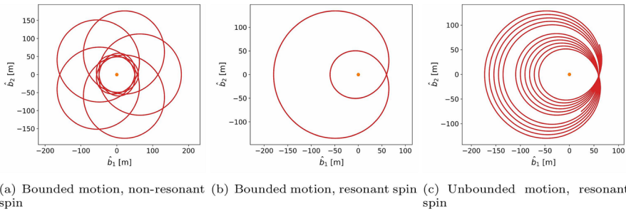
Fig. 3 In-plane trajectory shapes for an orbit-normal spin configuration
