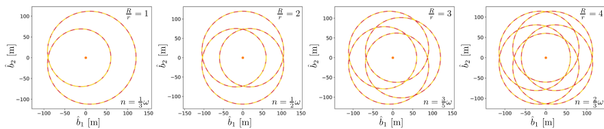
Fig. 9 Bounded body-frame relative trajectory for a circular chief orbit with orbit-normal spin motion, where spin rate is greater than orbit rate. The solid red curve is generated from the LROE formulation, while the dashed yellow curve is generated from the equivalent epitrochoid parameterization using the derived shape parameters
