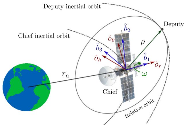
Fig. 2 Illustration of the Hill frame and Body frame: Spacecraft spinning about its radial axis
