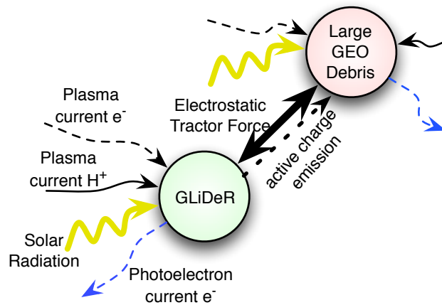
Figure 2. Balance of space environmental currents interacting with a spacecraft. The spacecraft equilibrium potential is obtained when the net current is zero.
