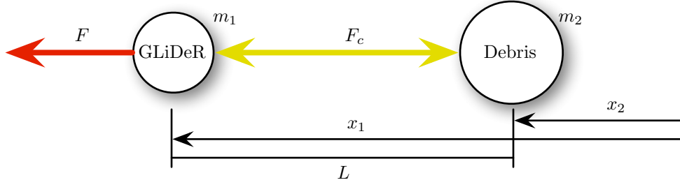
Figure 3. GLiDeR/Debris Force Diagram Illustration
