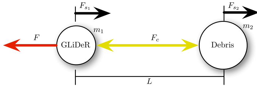
Figure 6. GLiDeR and debris force illustration with solar radiation pressure
