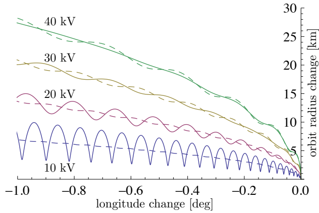
Figure 7. Orbit radius changes over a 1-degree longitude shift to move a 2000 kg debris object with (solid lines) and without (dashed lines) solar radiation pressure. Ticks indicate orbit completions, voltages are per vehicle.
