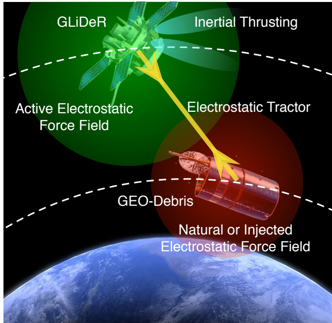
(a) Initial Approach to Geostationary Target
