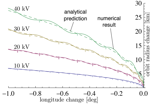
Figure 5. Orbit radius changes over a 1-degree longitude shift to move a 2000 kg debris object. Ticks indicate orbit completions, voltages are per vehicle.
