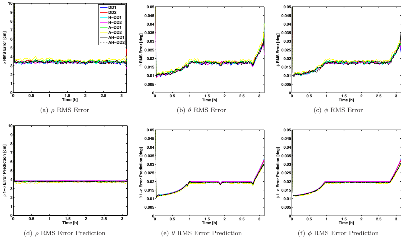
Figure 3. Gaussian Simulation Results: Position
