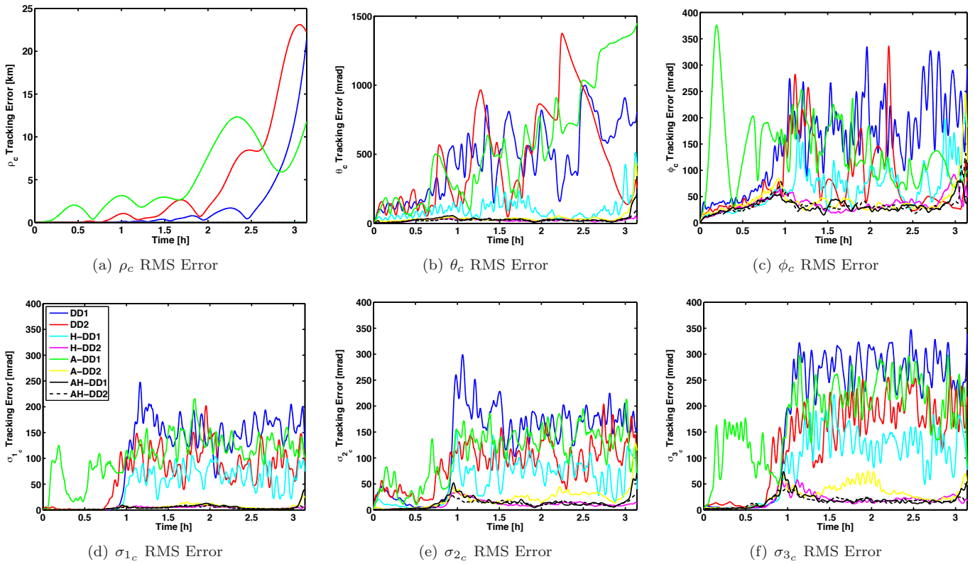
Figure 8. Non-Gaussian Simulation Results: Closed-Loop System Performance
