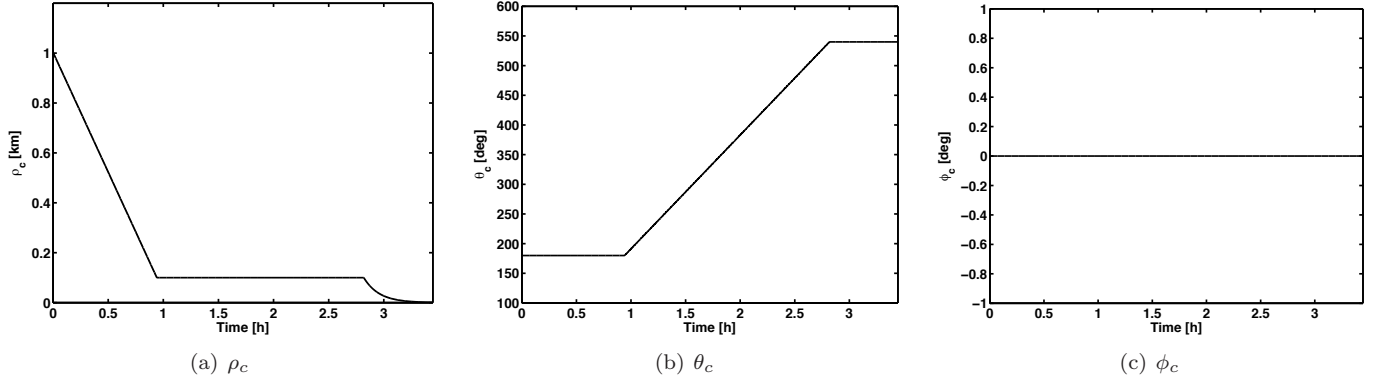
Figure 2. Guidance Commands
