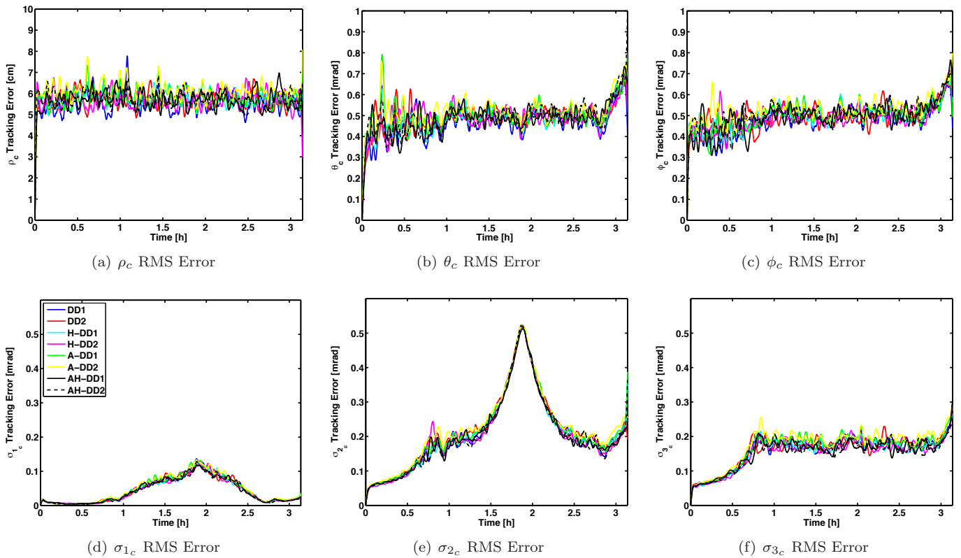
Figure 5. Gaussian Simulation Results: Closed-Loop System Performance
