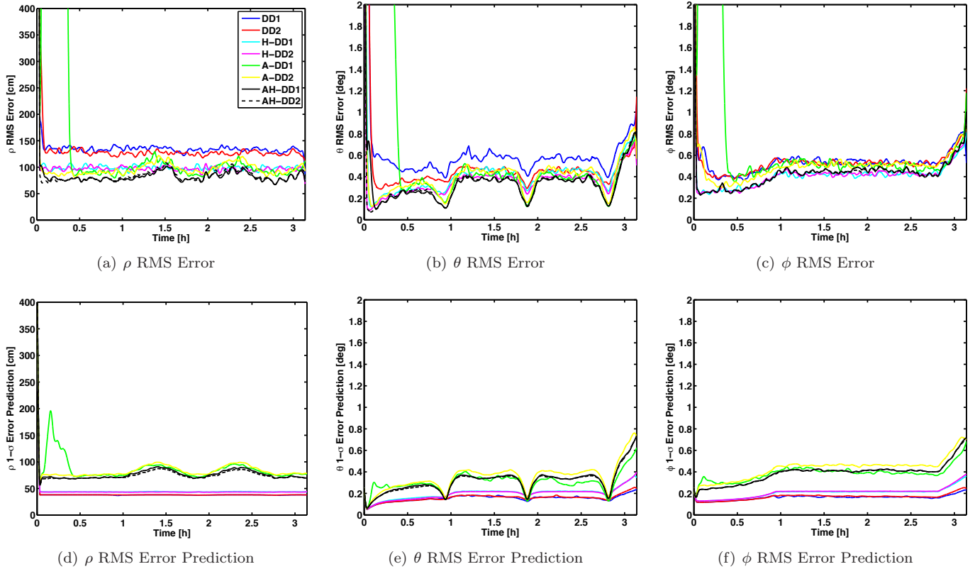
Figure 6. Non-Gaussian Simulation Results: Position
